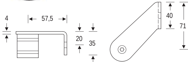
45° angle bracket Inward angled mounting strap Matt brushed stainless steel
