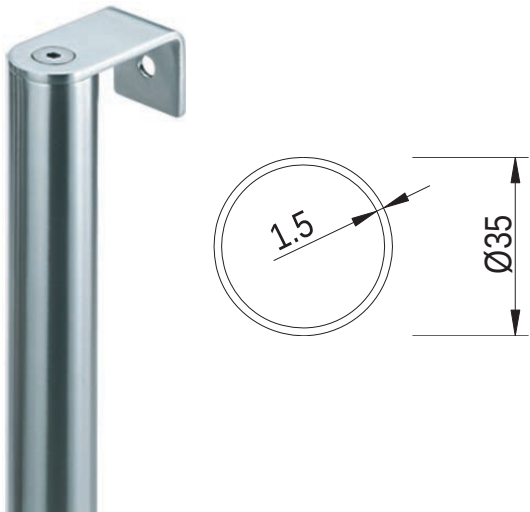
35mm diameter round tube (1.5mm thick) Matt brushed stainless steel
