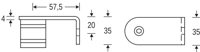
Straight bracket Inward angled mounting strap Matt brushed stainless steel
