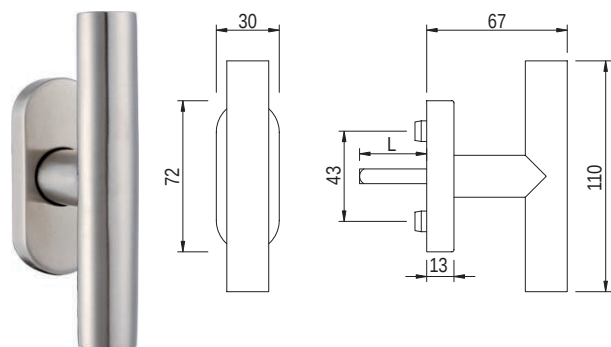
FG63L.ER T-Handle Non-Locking
